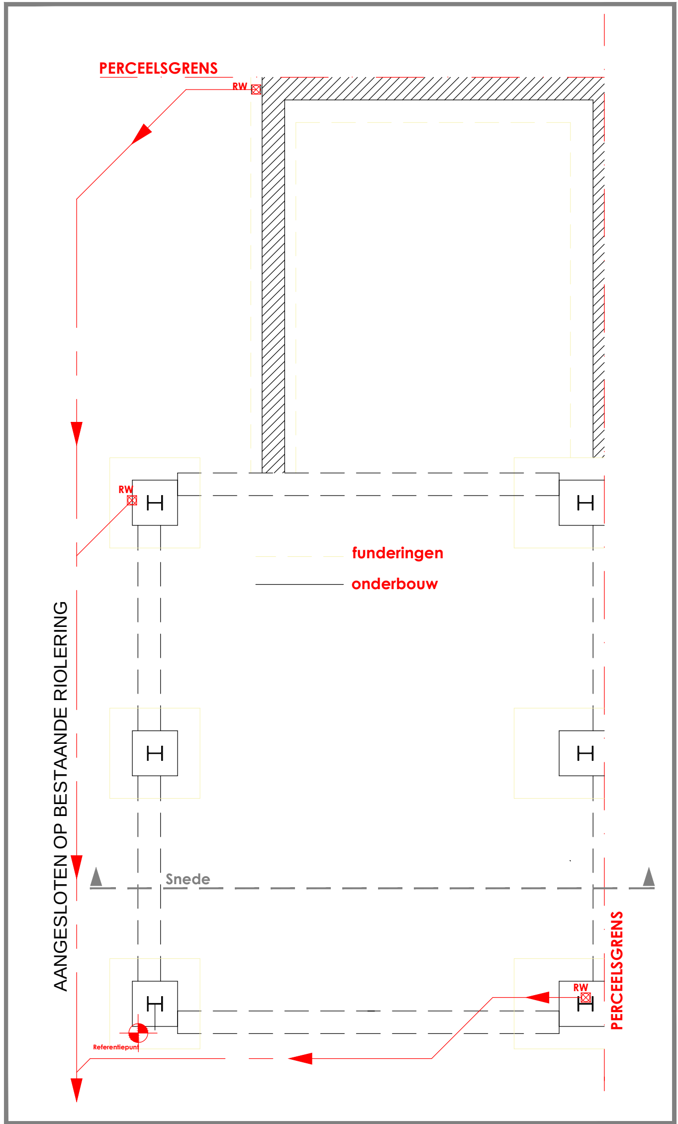
FUNDERING RIOLERING GARAGE / BERGING
