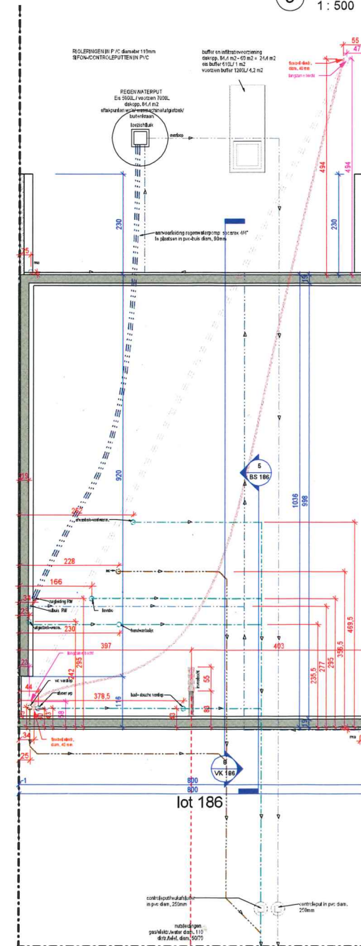
1 Riolering-fundering 186 VK 1: 50
